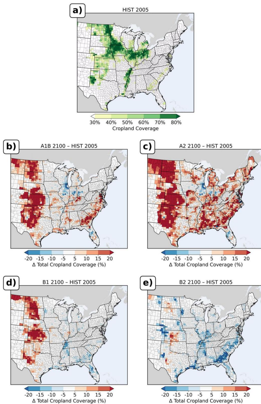
Fig. 4. As in Fig. 3, except for 2100.
