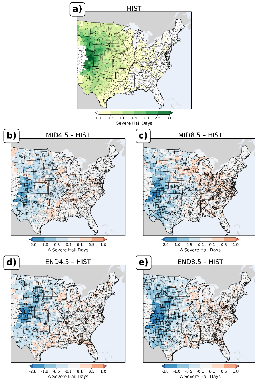
Fig. 8. a) HIST mean growing-season severe hail days and changes in mean growing-season severe hail days relative to HIST for b) MID4.5, c) MID8.5, d) END4.5, and e) END8.5. Counties with statistically significant differences between HIST and the future periods are denoted by thick black outlines ( p < 0.05 ; Mann-Whitney U test).
