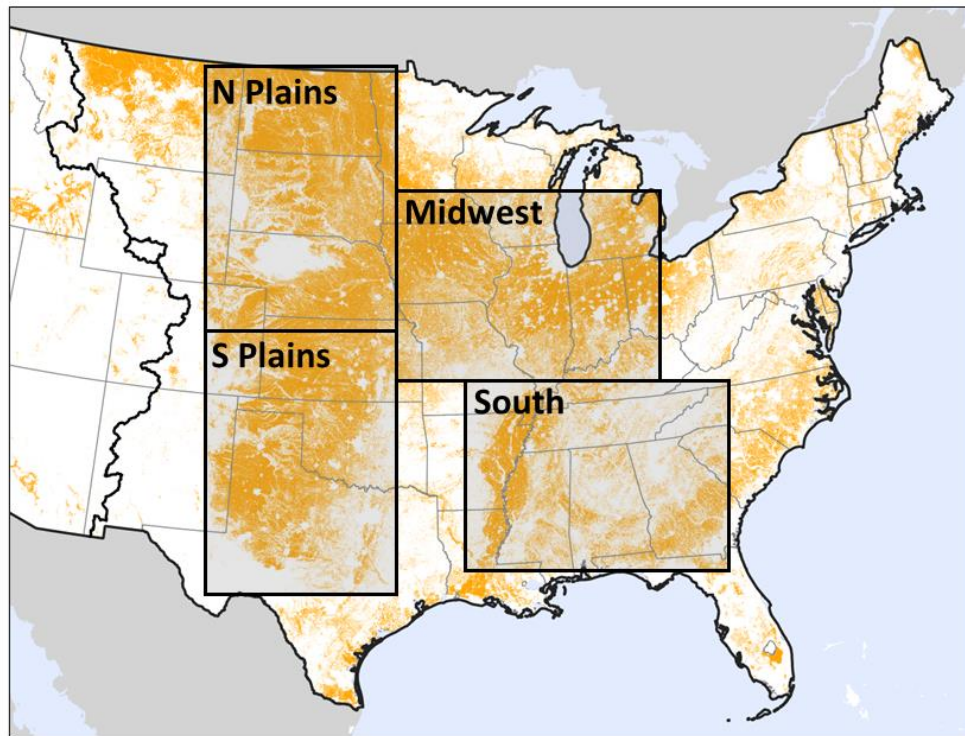
Fig. 1. Study domain with four equal-area study regions east of the U.S. Continental Divide. Cropland presence (cropland vs. non-cropland) from the A2 2100 scenario is displayed in orange at 250-m resolution.
