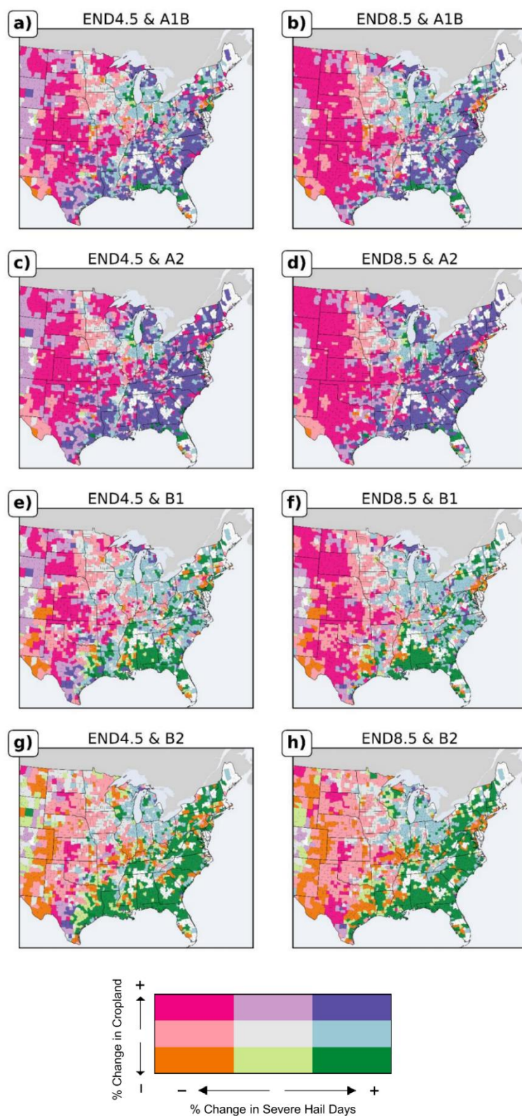
Fig. 10. As in Fig. 9, except for the end-of-century period.
