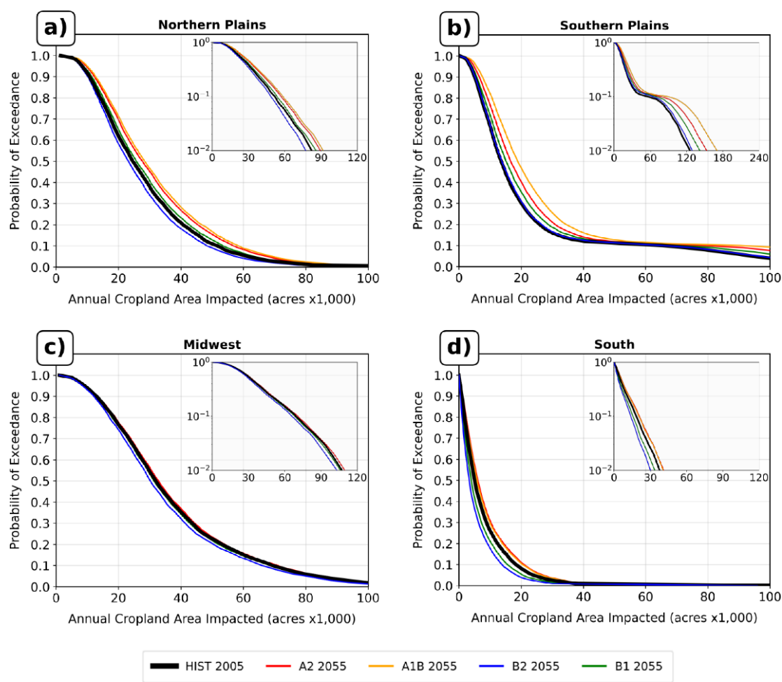
Fig. 6. Probability of exceedance (POE) curves comprising a 5,000-year HailMC simulation of the 2005 annual cropland area impacted by severe hail (solid black line), the 2055 annual cropland area impacted by severe hail for each IPCC SRES scenario (A1B, A2, B1, B2) by region: a) Northern Plains, b) Southern Plains, c) Midwest, and d) South. Each panel contains a subplot of the same POE curves with a log (y) axis.
