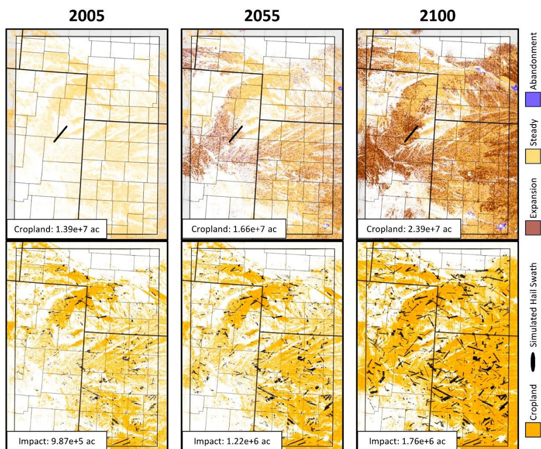
Fig. 5. Example HailMC simulation over eastern Colorado, western Kansas, and western Nebraska showing historical (2005) and projected A2-scenario cropland exposure surface for 2055 and 2100. Top panels show cropland extent for each period, with cropland expansion relative to 2005 displayed in red and cropland abandonment in blue; the black line denotes a single example simulated hail swath. Bottom panels display cropland (orange) and hail swaths (black) simulated using 500 years drawn from the 5,000-year HailMC simulation, with swaths shaded by their relative cropland impact (darker swaths indicate greater impact). Insets report total cropland area in the top panels and total impacted cropland area in the bottom panels.
