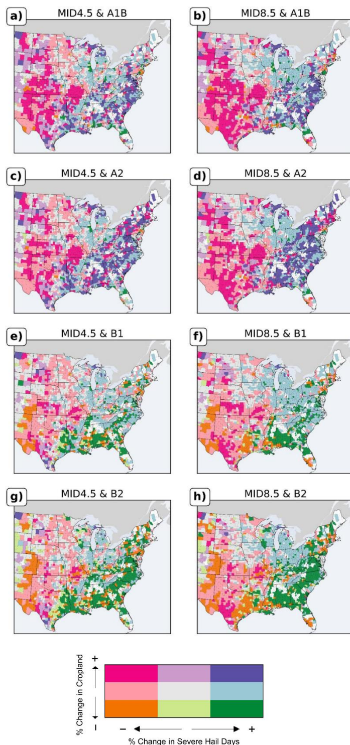
Fig. 9. Bivariate county-level changes in severe hail days paired with cropland coverage for mid-century WRF-BCC climate simulations and 2055 IPCC SRES cropland scenarios: a) MID4.5 & A1B, b) MID8.5 & A1B, c) MID4.5 & A2, d) MID8.5 & A2, e) MID4.5 & B1, f) MID8.5 & B1, g) MID4.5 & B2, and h) MID8.5 & B2. Colors represent the combined direction and magnitude of percent change in severe hail days and cropland coverage relative to historical conditions. Positive (negative) percent changes refer to severe hail-day or cropland changes > 20\% ( < -20\% ).
