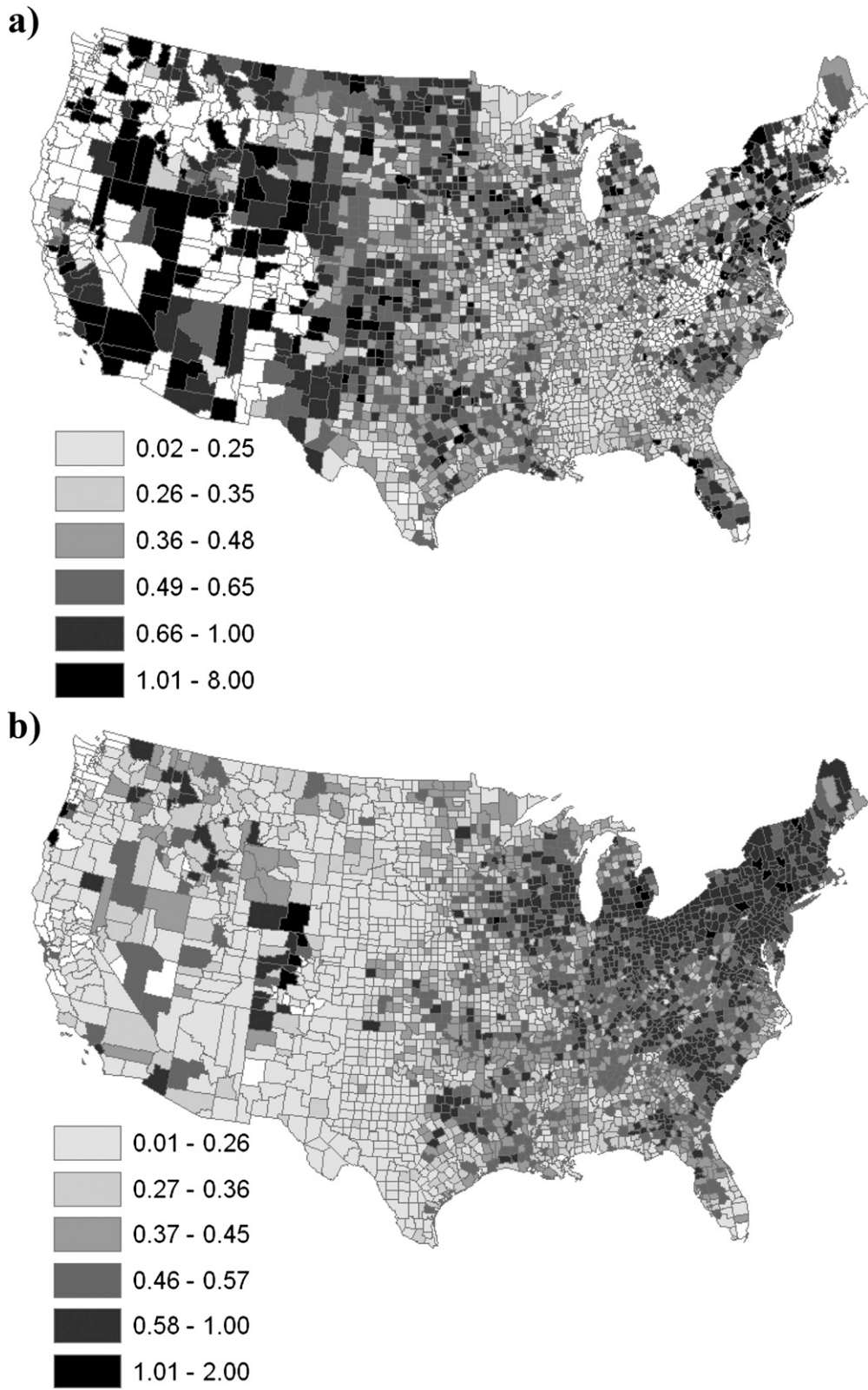
FIG. 5. Ratio of (a) tornado reports divided by tornado warnings per county, 1986–2007; and (b) combined nontornado convective wind reports and hail reports divided by severe thunderstorm warnings per county, 1986–2007.
